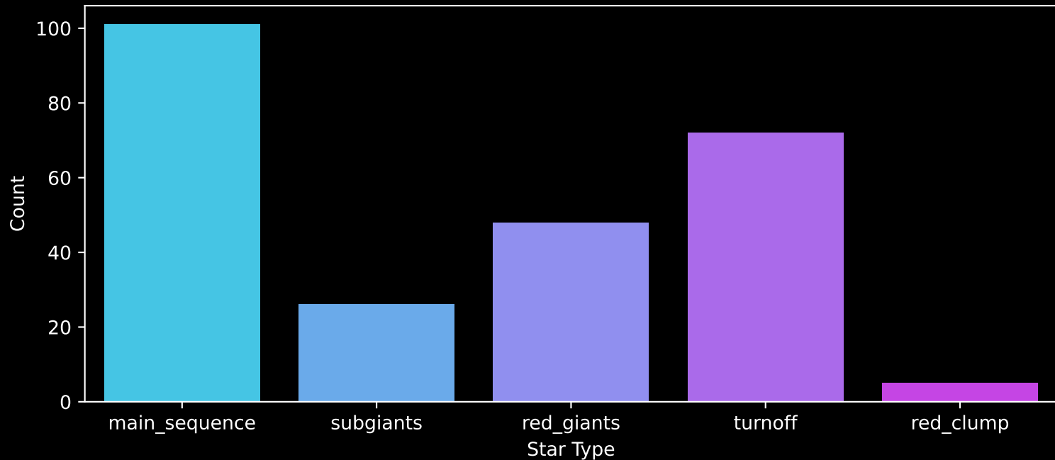
GALAH DR4 Field: [3237] Count plot of Star Type
