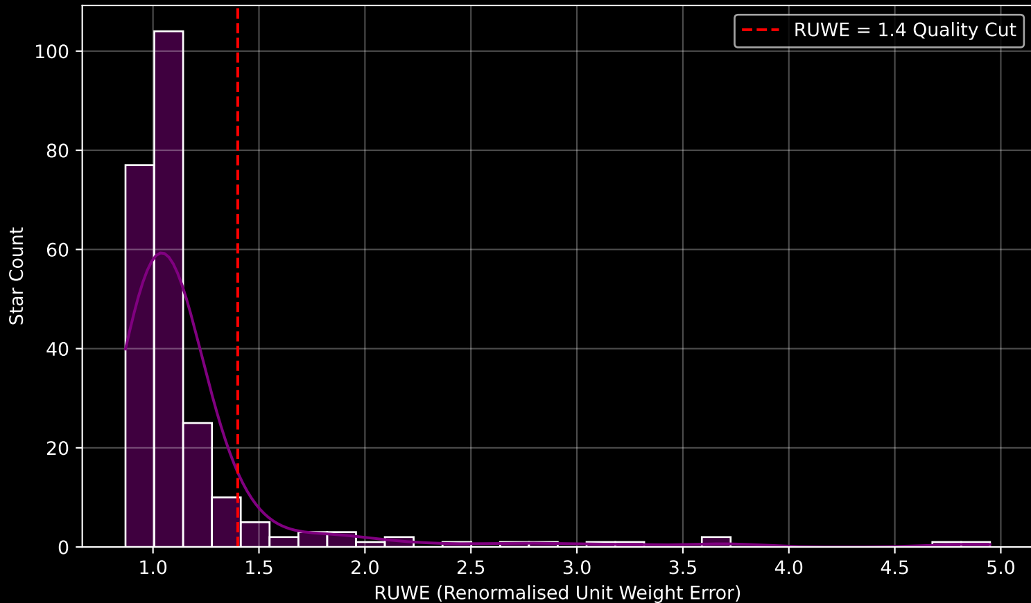
GALAH DR4 Field [3237] RUWE Distribution (n= 241)
