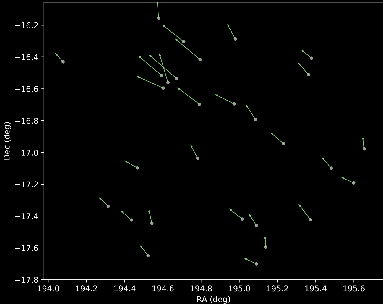
GALAH DR4 Cluster 5 Proper Motion Vectors (n=29)
