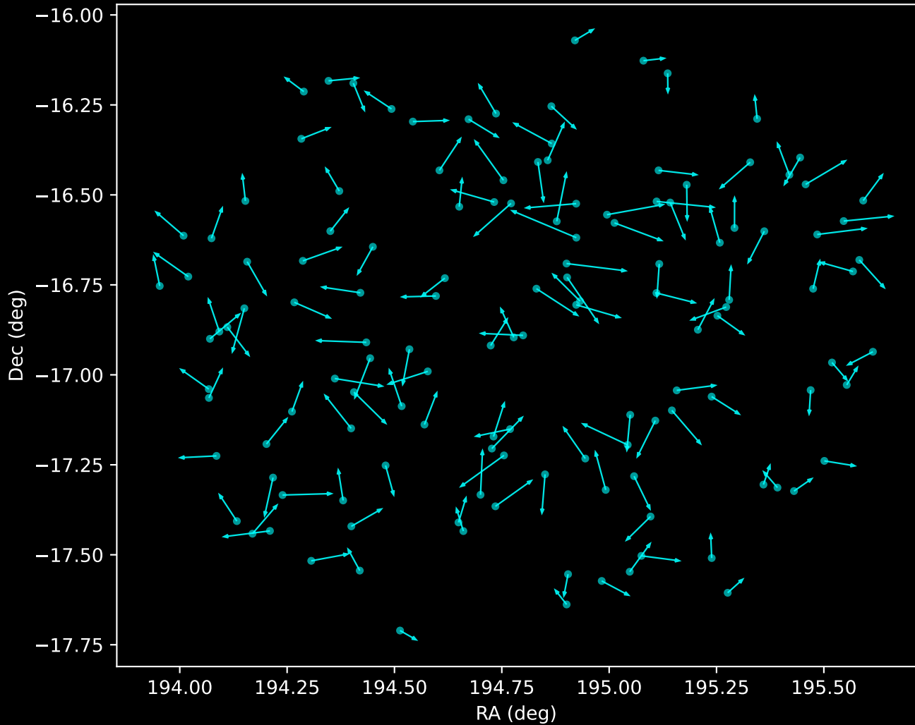
GALAH DR4 Noise Stream Proper Motion Vectors (n=134)
